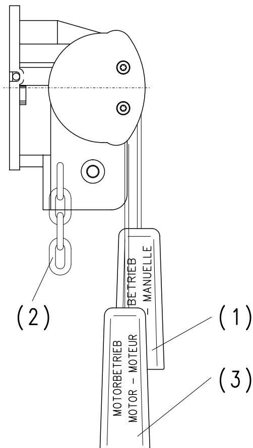
Fig. 1: Noodhandbediening "Snelle-Ketting"
